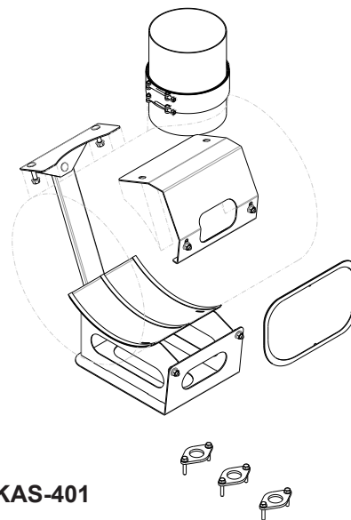
Adaptor kit for Claas Lexion 7000 & 8000
