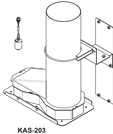
Adaptor kit for Case 4WD Tractors w/ circular intakes
