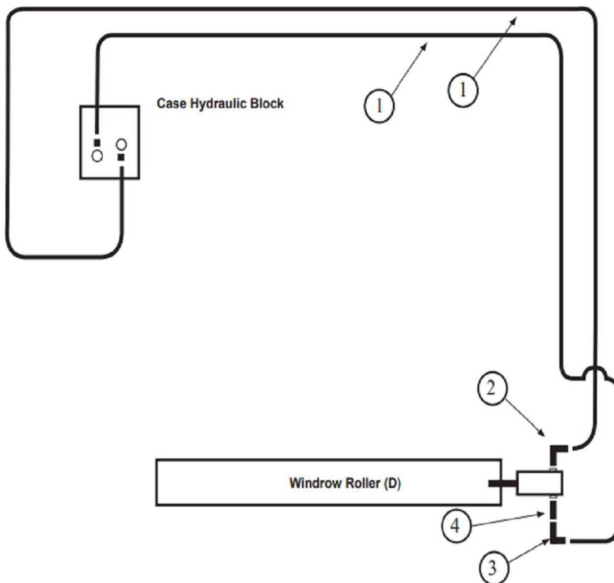
SCU & Windrow Hydraulic Schematic
