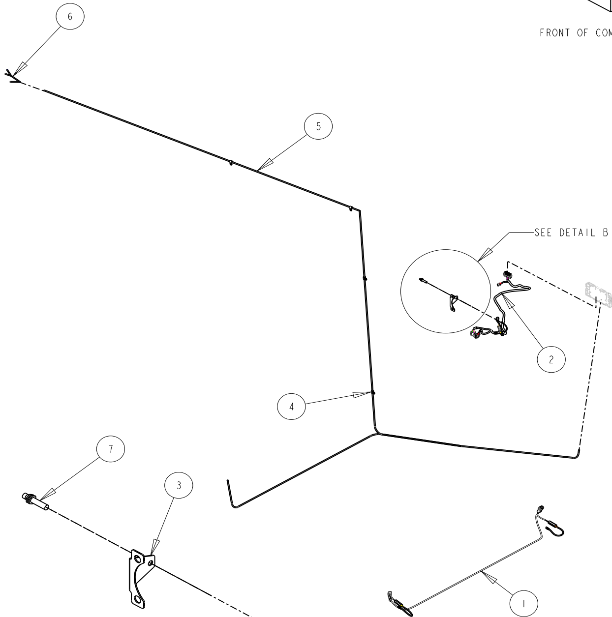
DETAIL B
