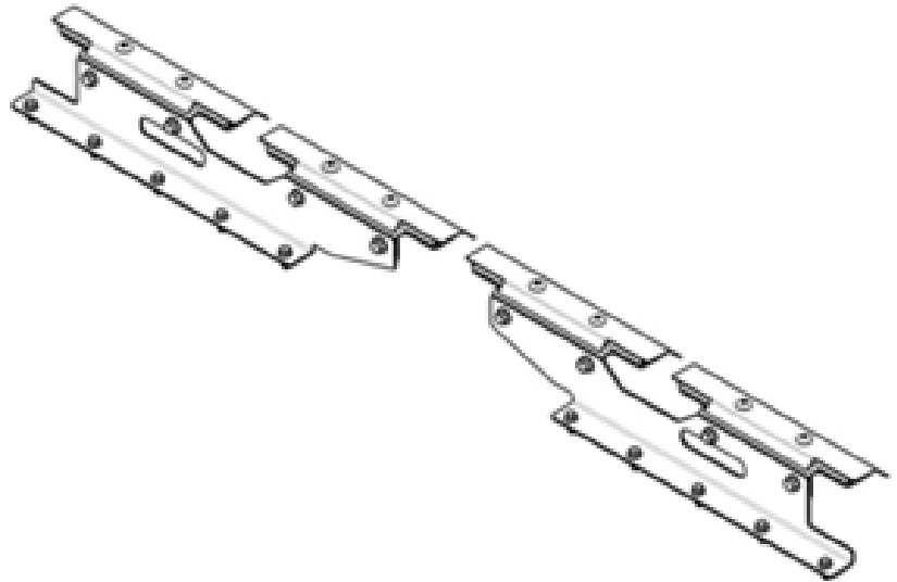
Product Number: 850-104 S600 Magnet Kit
